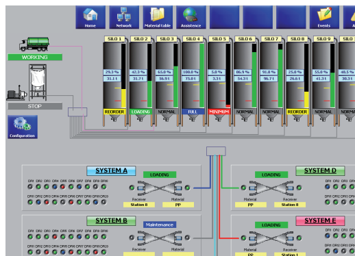
Silo loading
